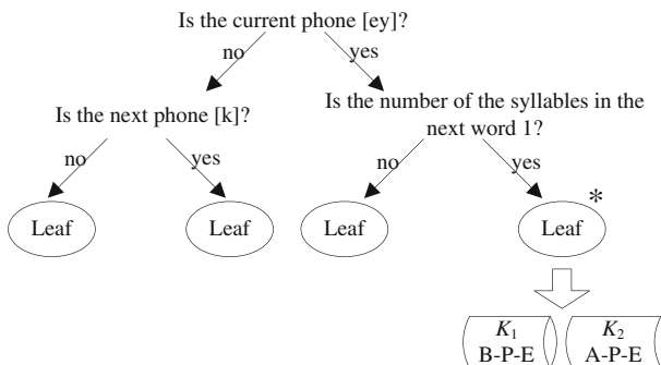
Fig. 3 Part of the decision tree for generating f_0 . Data is available for only two emphasis categories B-P-E ( K_1 ) and A-P-E ( K_2 ) in the leaf node annotated by ‘‘*’’. There are four phones in K_1 : [ey][ow][ae][ch] and two phones in K_2 : [m][n]
