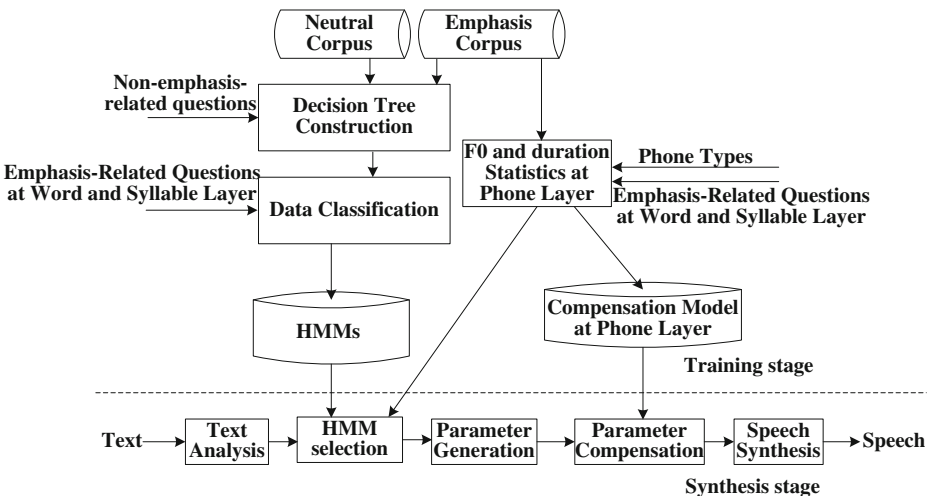
Fig. 2 Diagram of the model for emphatic speech synthesis with hidden Markov model
